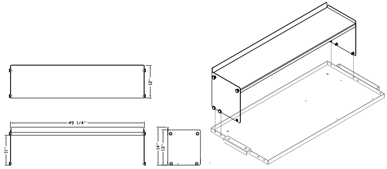
Mag Senior Sound Tray with Mag 24" Top Shelf
