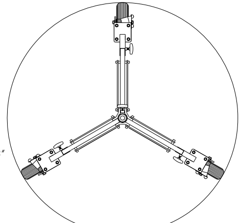
53 7/8" Diameter Circle
