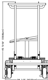
Cable X-Over Cart shown with optional (Aluminum) Folding Plate
