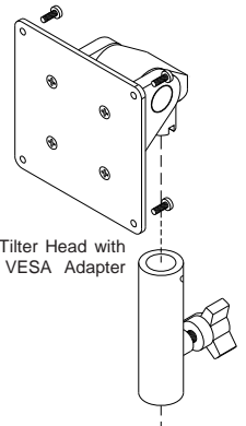
Mag LCD 4" Tilt Head Pin Adapter
