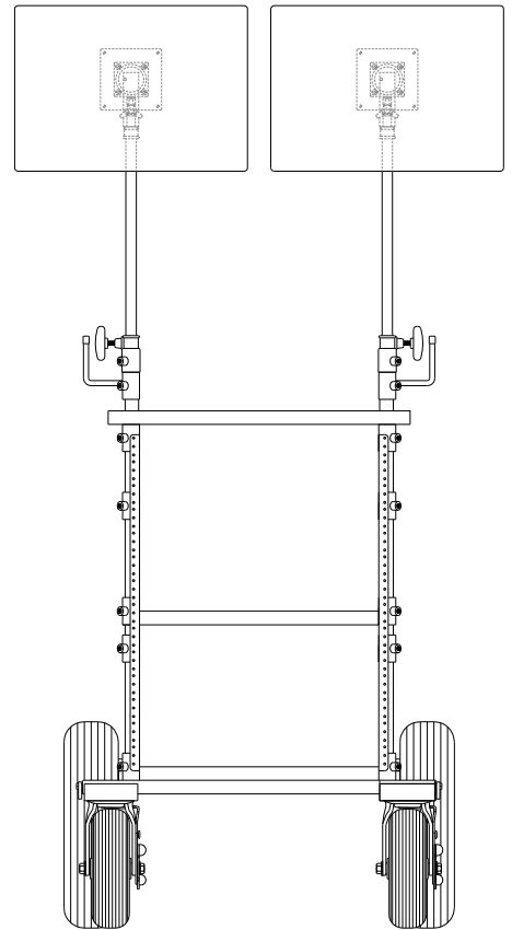
TR-01 8 shown with (2) TR-01 VPR units, includes the following accessories: (MAG-LCD TH-LD BK) Mag LCD Tilter Head with 75/100mm VESA Adapter Plate (3-24 lbs.) (2) (MAG-LCD MR-04) Mag LCD 4" Tilt /Head Pin to 5/8" Baby Pin Adapter. (2) (MAG-01 VPR-B ST) Mag Baby Pin Extension Riser (Steel) (2) (TR-01 Z) VPB Adapter to Mag Baby Pin Riser (2)
